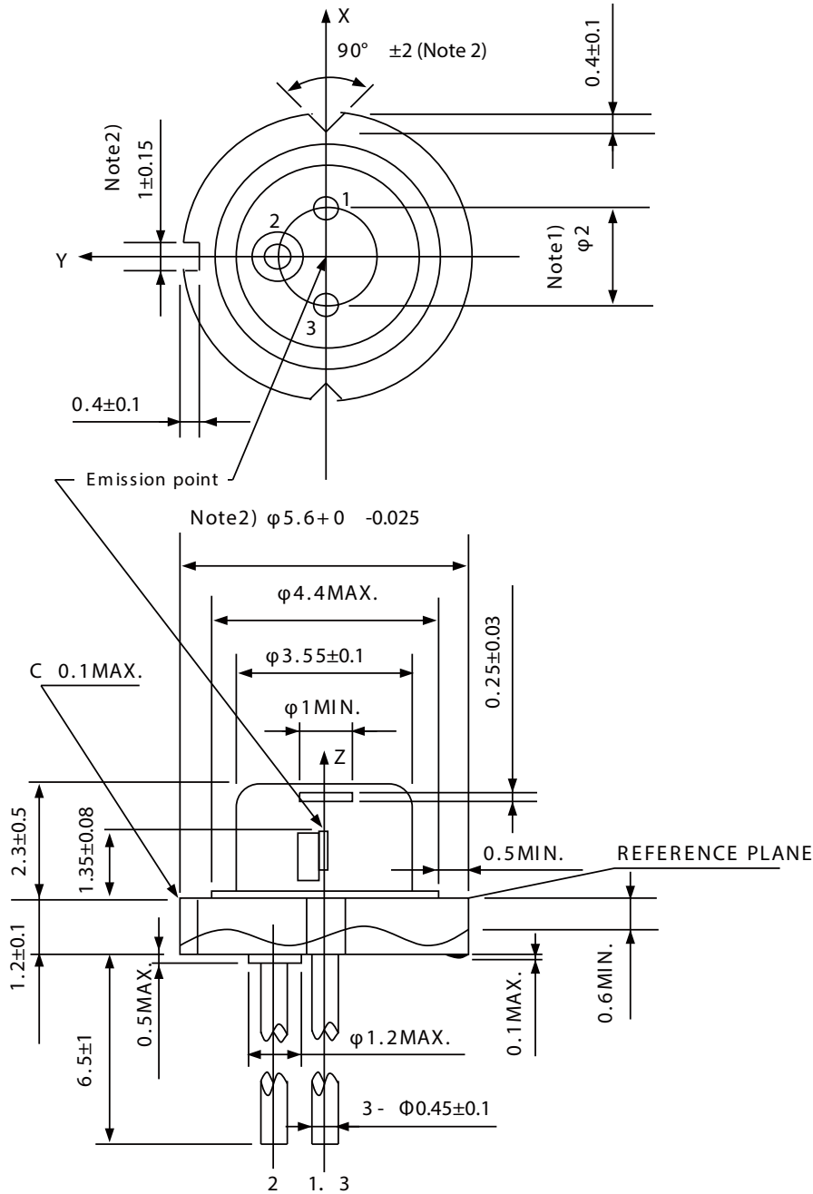
Outline dimensions and Terminal connections
